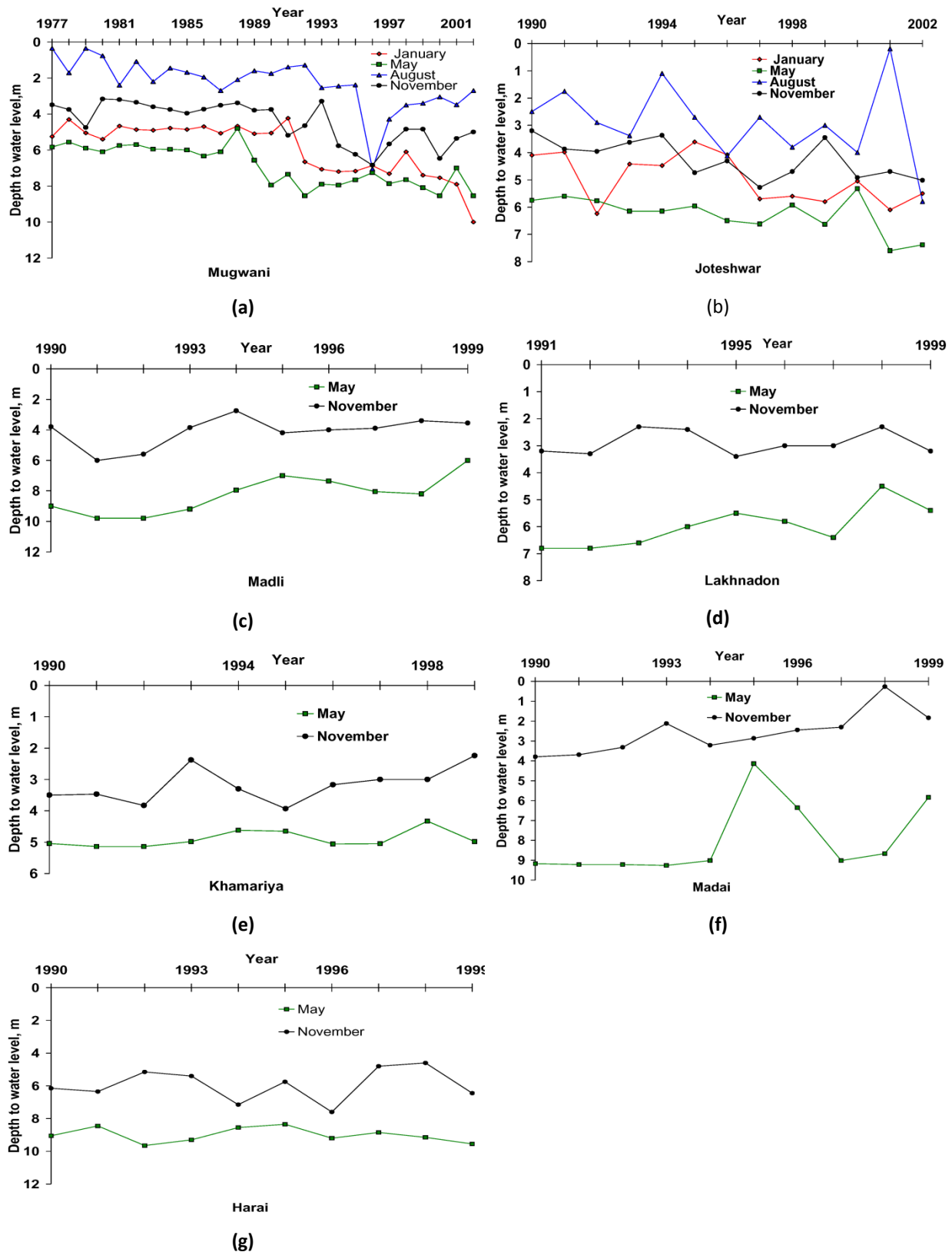
Figure 6: Depth to ground water table fluctuations over the years in hard geological formations (Gondwana and Deccan trap)
