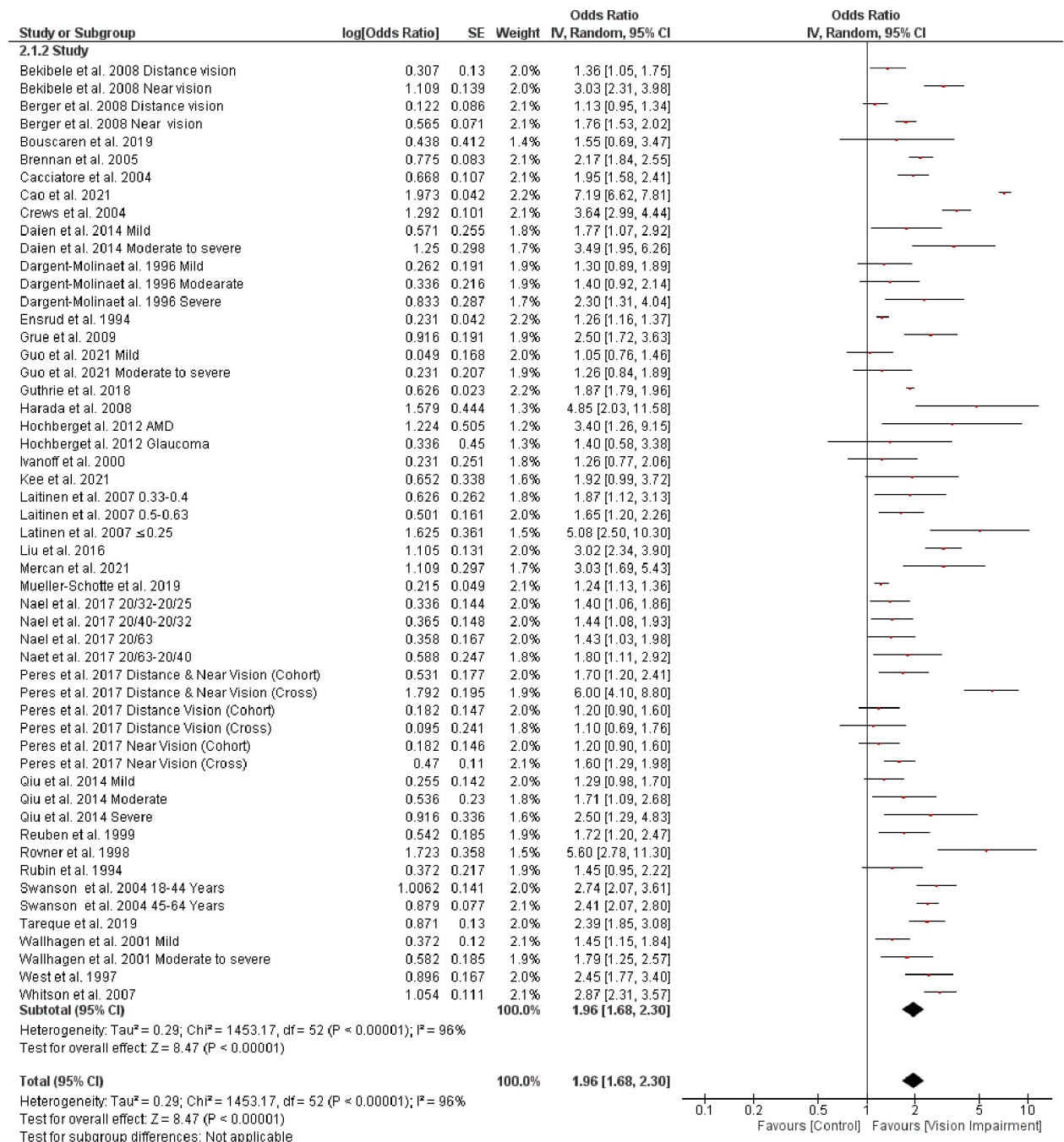
Fig 10. Forest plot of the association between vision impairment and difficulties with instrumental activity of daily living.
